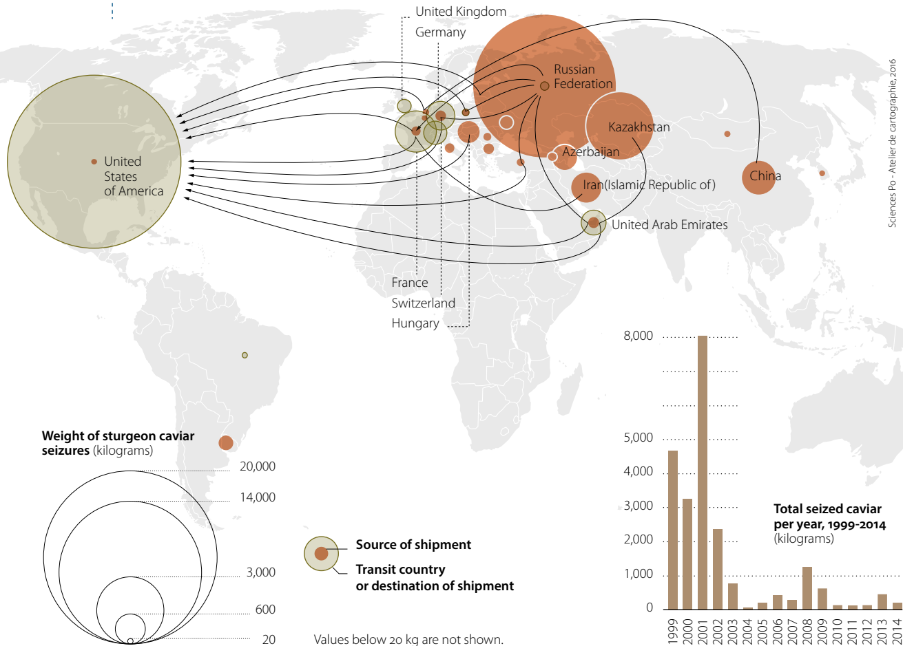
Map 1 Main flows of sturgeon caviar seizures (kg), 1999-2014
