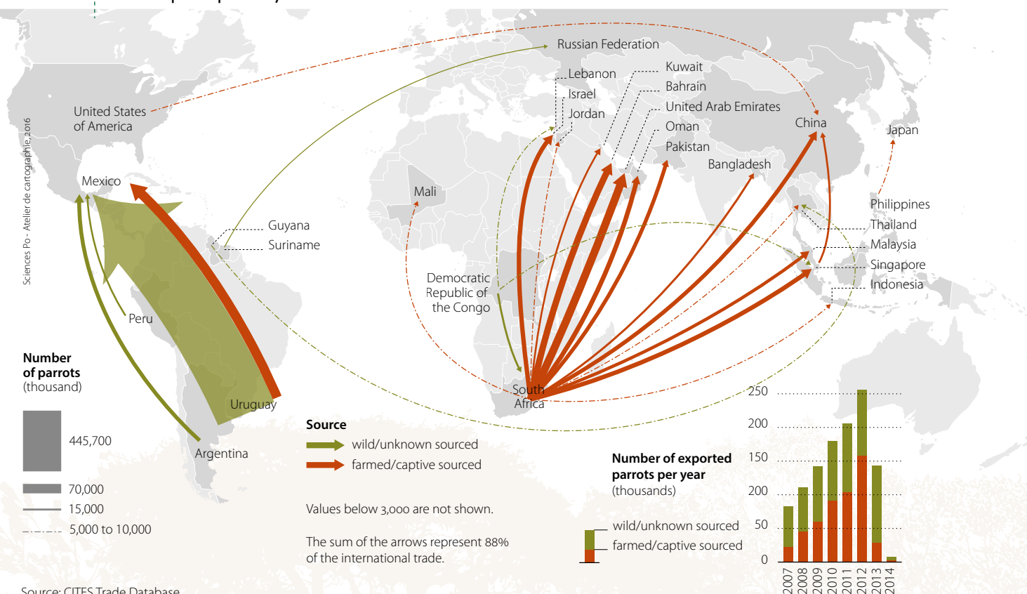
Map 2 Main flows of legal trade in parrots based on CITES permits, 2007-2014 (New world and Afro-tropical parrots)
