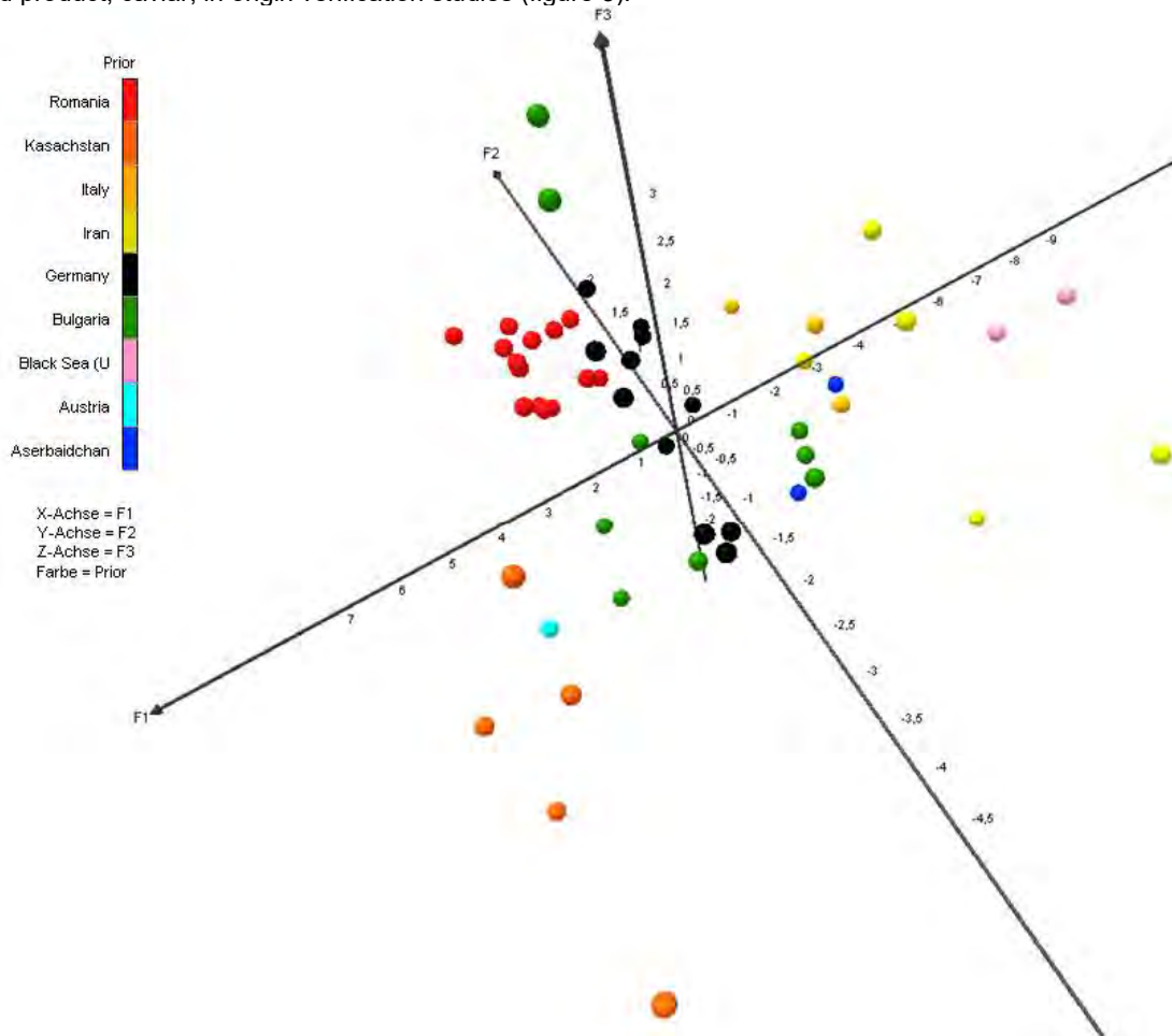
Figure 3: Agroisolab Database of sturgeon: D/H and ^{18}\text{O}/^{16}\text{O} isotopic ratio of the tissue water and the organic fraction.
